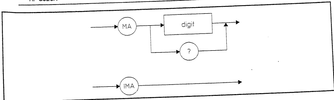
Figure 2-25. MA Syntax Diagram
